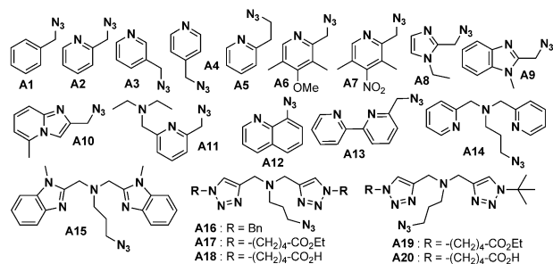
Scheme 3. Structures of azides A1–A20 .
