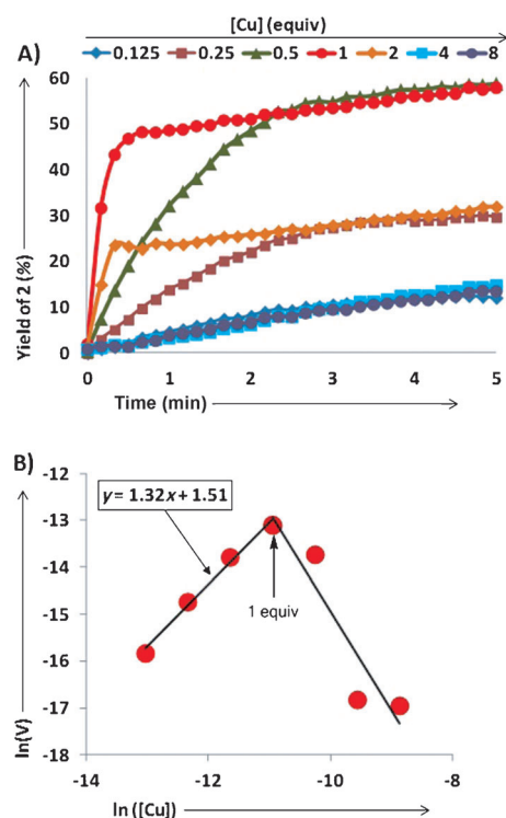
Figure 2. A) Time courses for various concentrations of [\text{CuSO}_4 \cdot \text{H}_2\text{O}] . [\text{I}] = [\text{A20}] = 17.5\ \mu\text{M} . B) Determination of the reaction order in copper.
